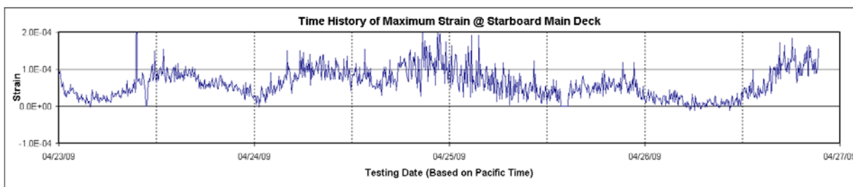
FIGURE 5 Sample Recordings of Strain at Port Main Deck (Extreme Value in 5 Minutes)
