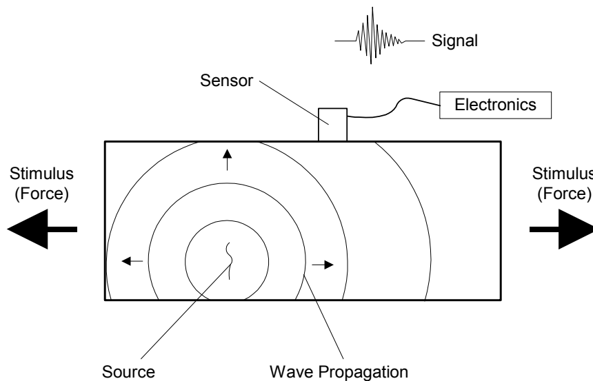
FIGURE 1 Schematic of the Acoustic Emission Process
