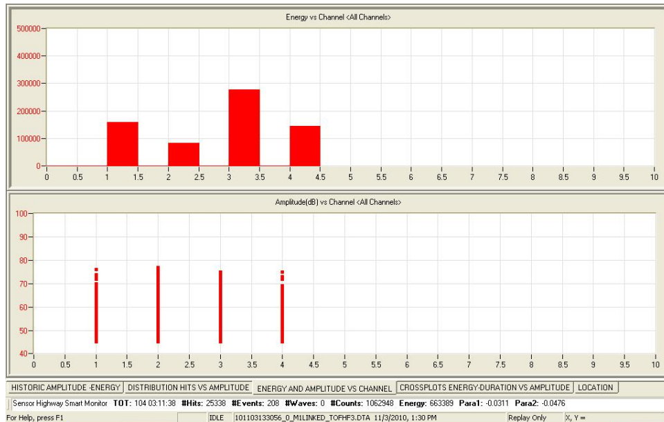
FIGURE 9 Cross Plot: Energy and Amplitude versus Channels
