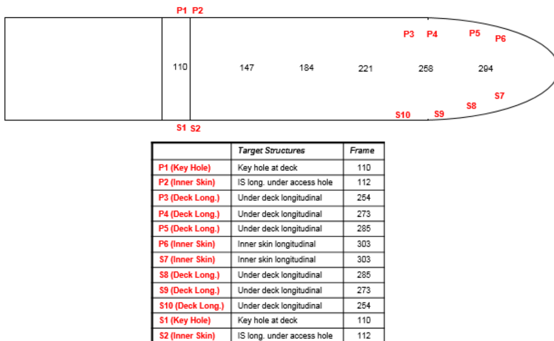
FIGURE 2 Selected Areas That May be Prone to Cracking
