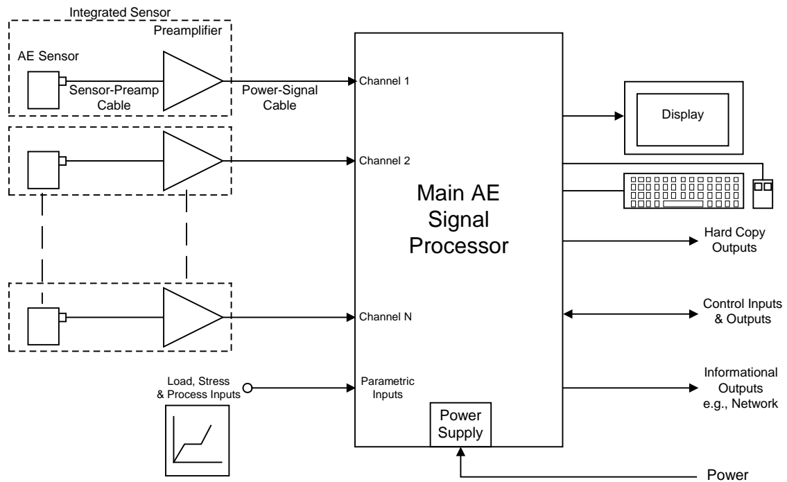
FIGURE 1 Acoustic Emission System Block Diagram
