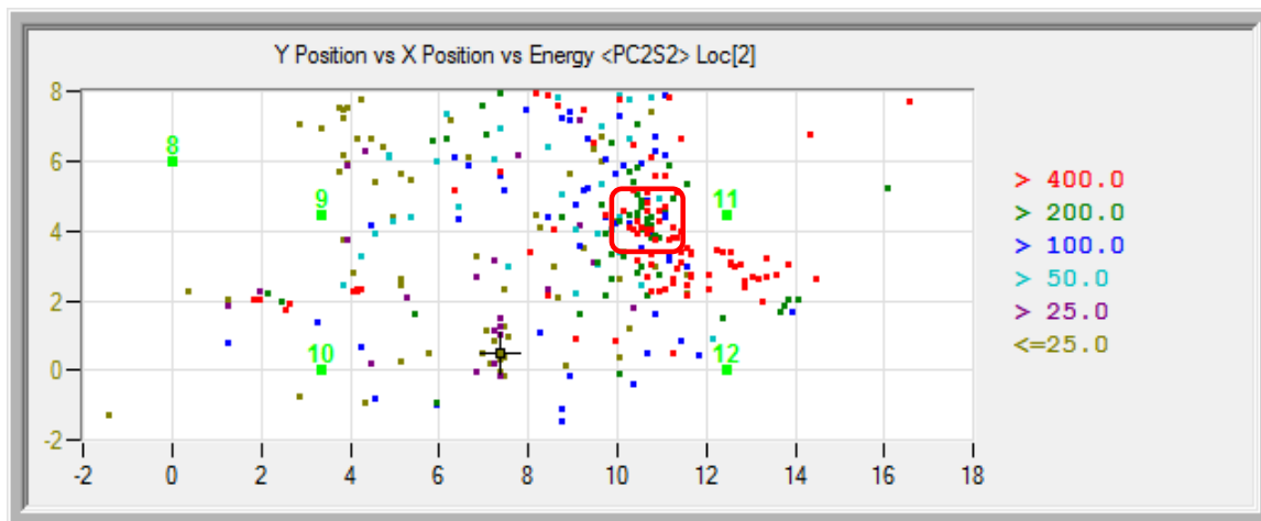
FIGURE 3 Source Location Cluster Formed During Ocean Voyage
