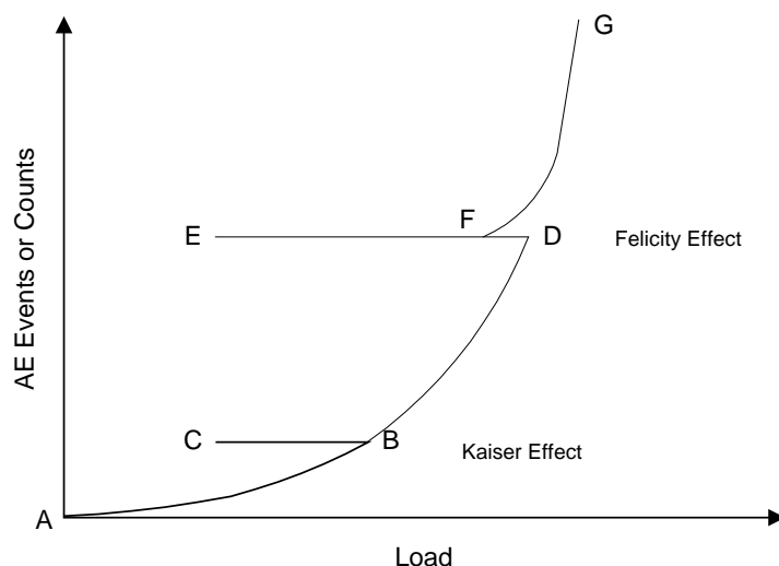
FIGURE 3 Emission on Repeated Loading
