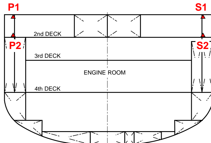
FIGURE 3 Arrangement of Strain Gauges for Hull Monitoring System
