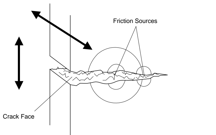
FIGURE 4 Indication of Crack Face Rubbing
