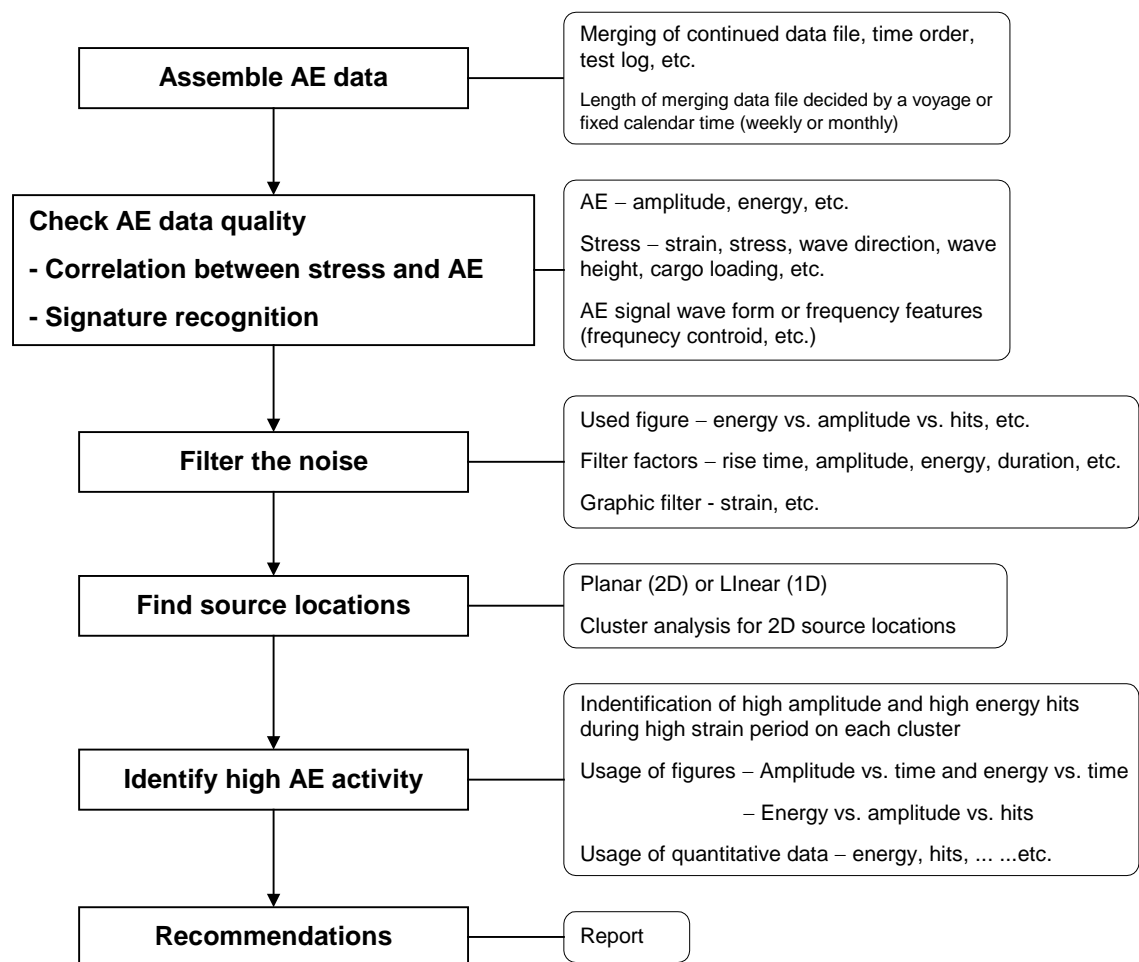
FIGURE 1 Procedure for Data Analysis
