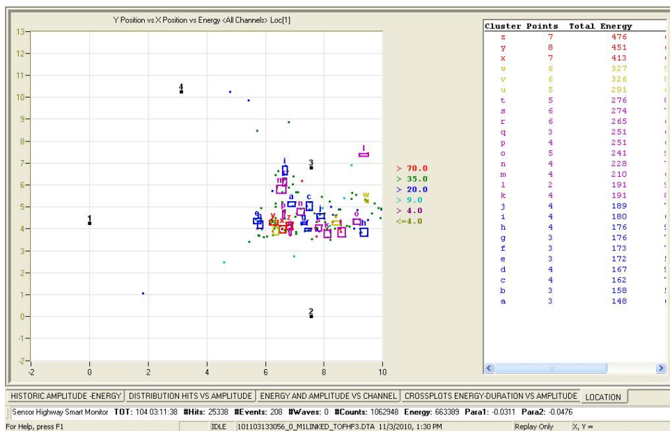
FIGURE 11 Clusters in the Zonal Source Location
