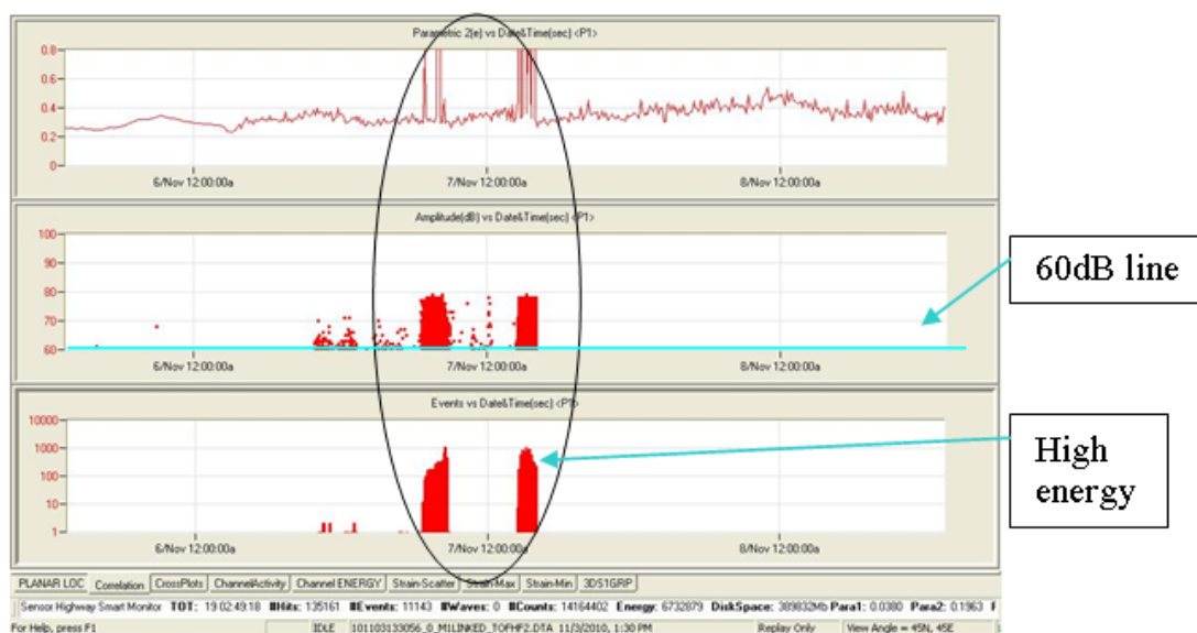
FIGURE 7 Correlation between Stress and Acoustic Emission
