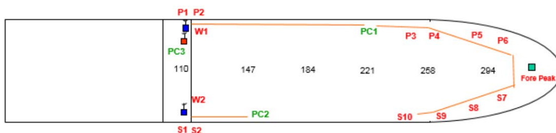
FIGURE 6 Layout of Acoustic Emission Sensors and Computers
