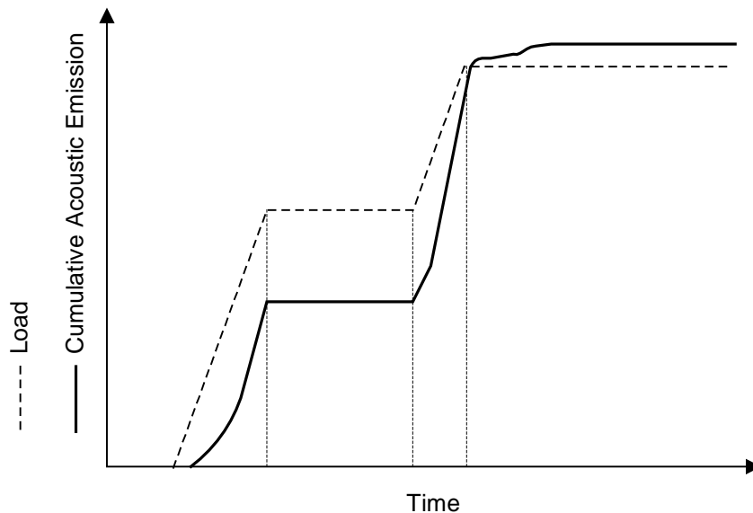
FIGURE 2 Emission Instability
