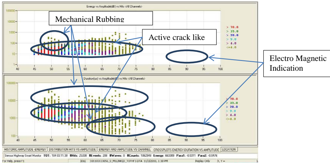
FIGURE 10 Cross Plot: Energy and Duration versus Amplitude
