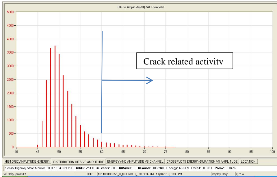
FIGURE 8 Cross plot: Number of Acoustic Emission Hits versus Amplitude
