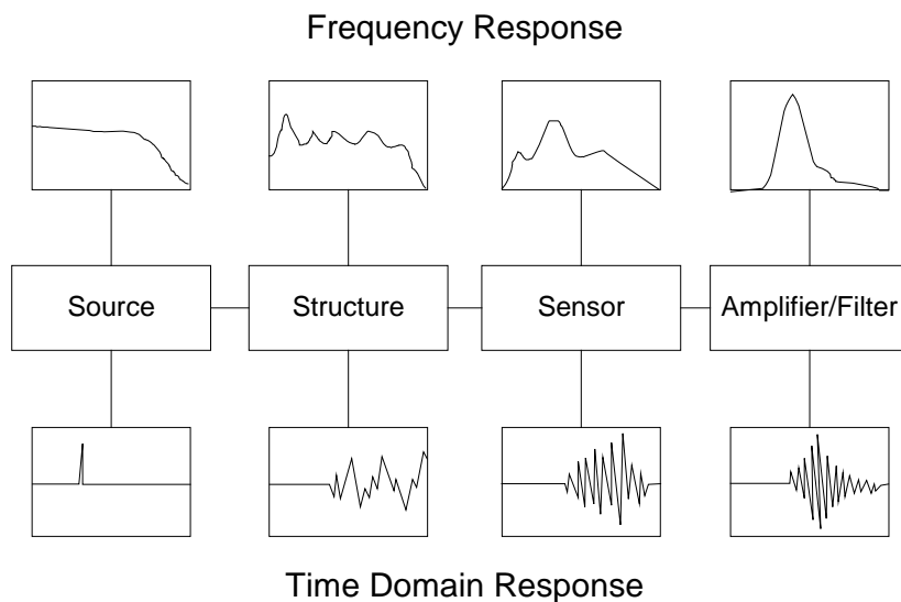
FIGURE 5 The Signal Formation Chain
