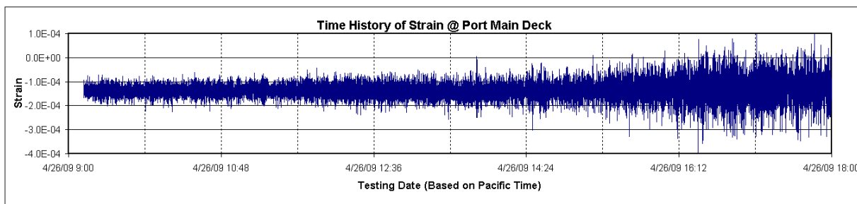
FIGURE 4 Sample Recordings of Strain at Port Main Deck (Raw Data)
