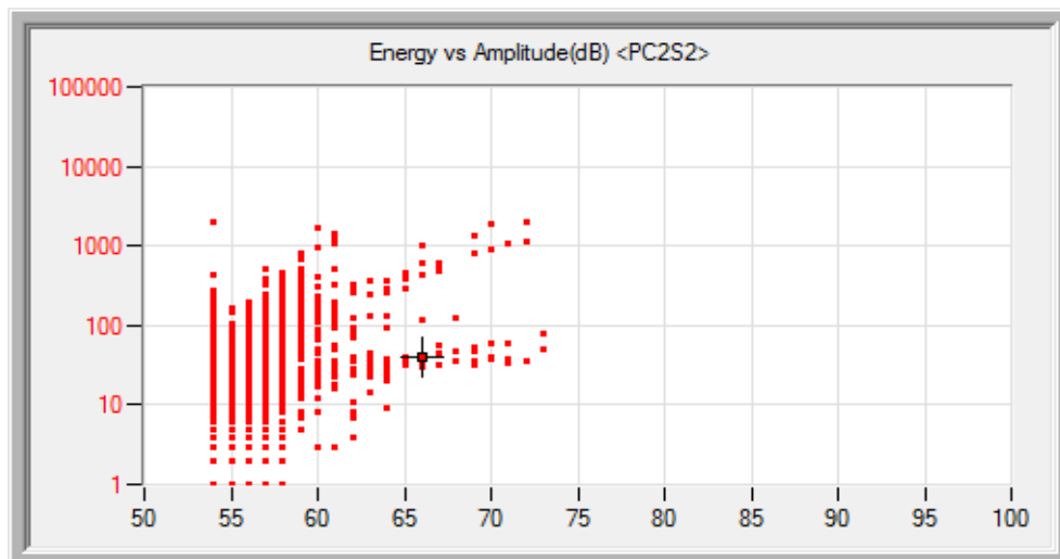
FIGURE 2 An Example of the Energy vs. Amplitude Cross Plot
